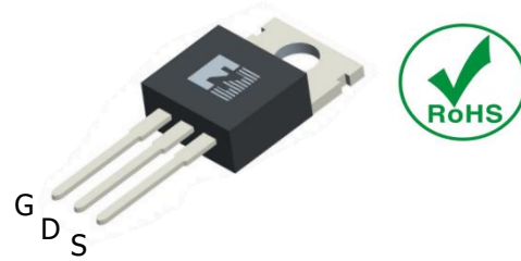
TO-220
